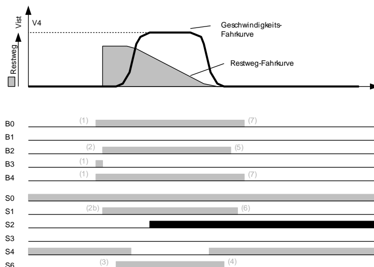
Abbildung 9-2: "Vorwarn"-Bit
