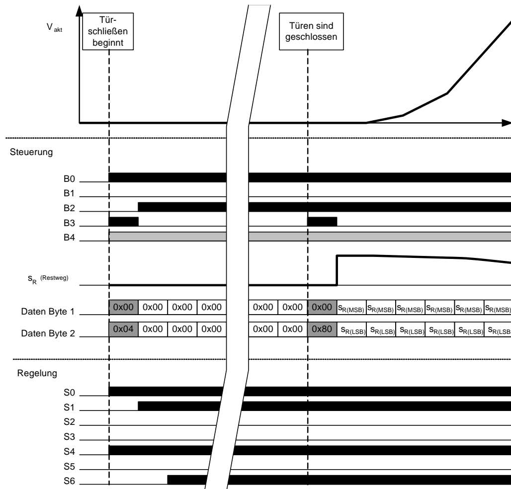
DCP4: Start-Sequenz "Schnellstart"
