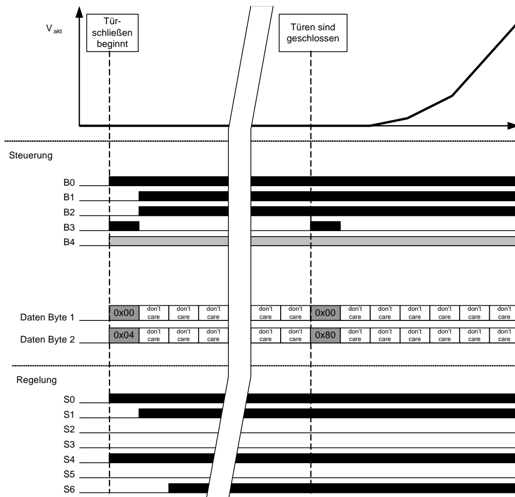
DCP3: Start-Sequenz "Schnellstart"
